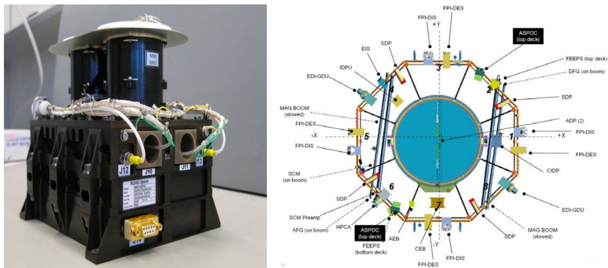
Figure 2-1 ASPOC Instrument Picture and Spacecraft Accommodation
