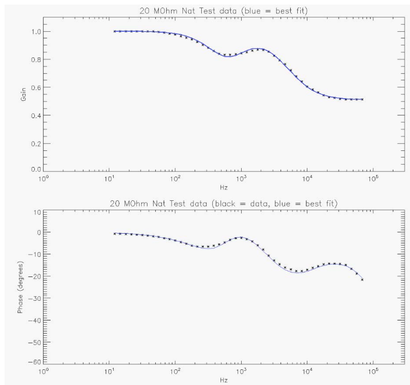
Figure 11-14 Gain and Phase Correction Applied to ADP
