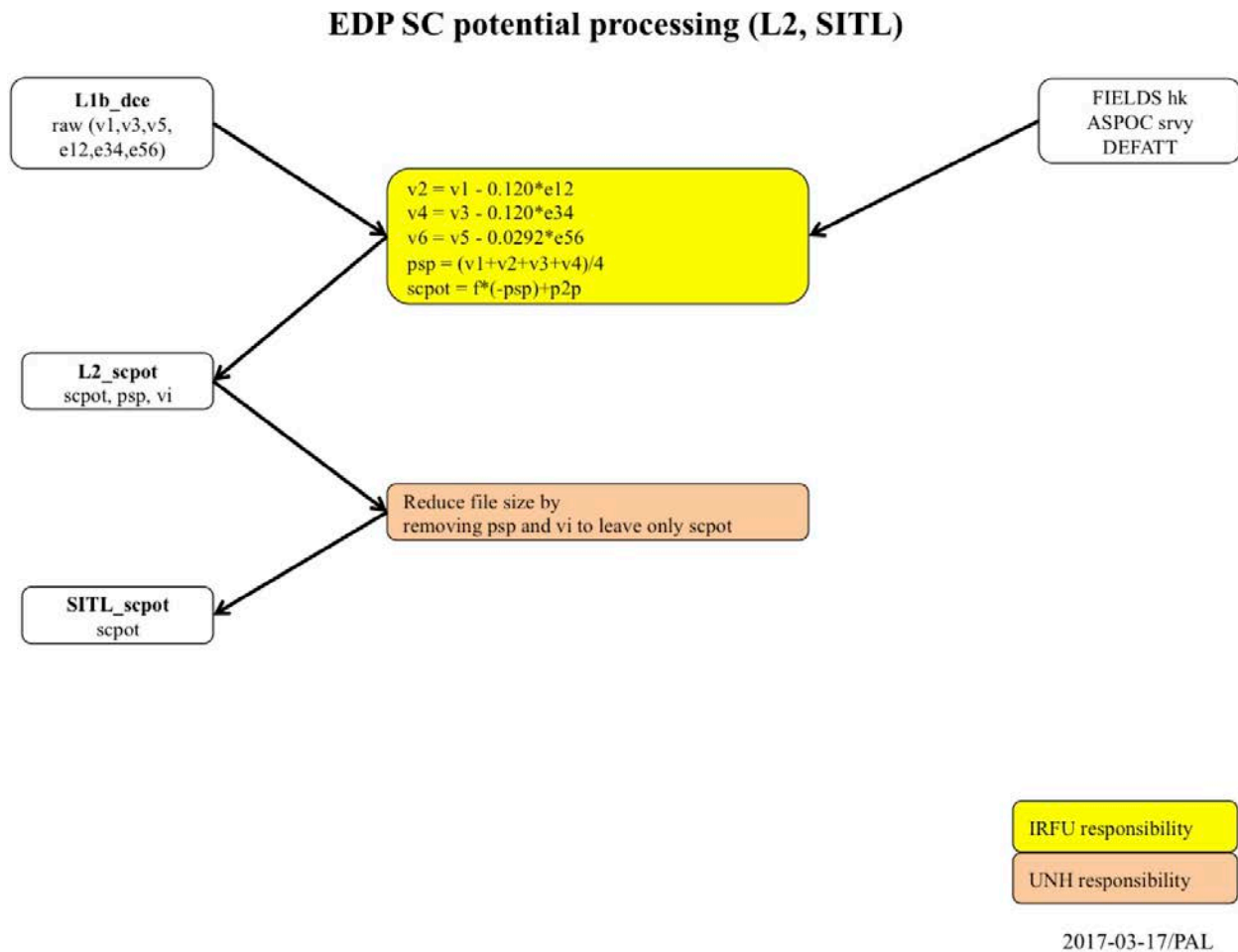
Figure 11-17 Flow diagram of EDP Level 2 and SITL Spacecraft potential processing
