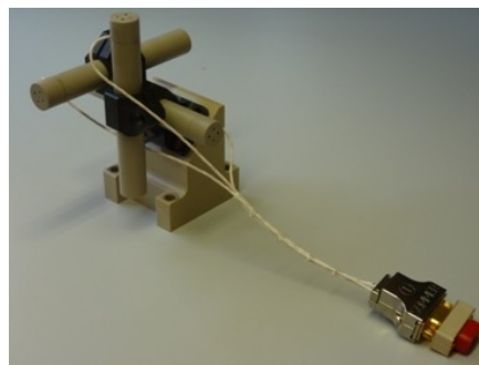
Figure 9-1 SCM Sensor
