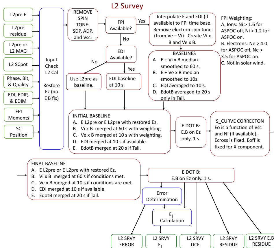
Figure 11-10 L2 Calibration Algorithm
