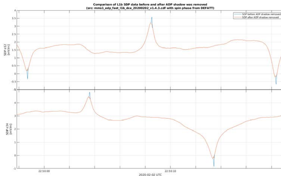
Figure 11-6 Example of Removed ADP Shadow from the SDP E-Field Measurements (e12 and e34). Data taken from mms1_edp_fast_l1b_dce_20200202_v1.4.3.cdf and just after the ADP shadow was removed, thus it is still in instrument frame.
