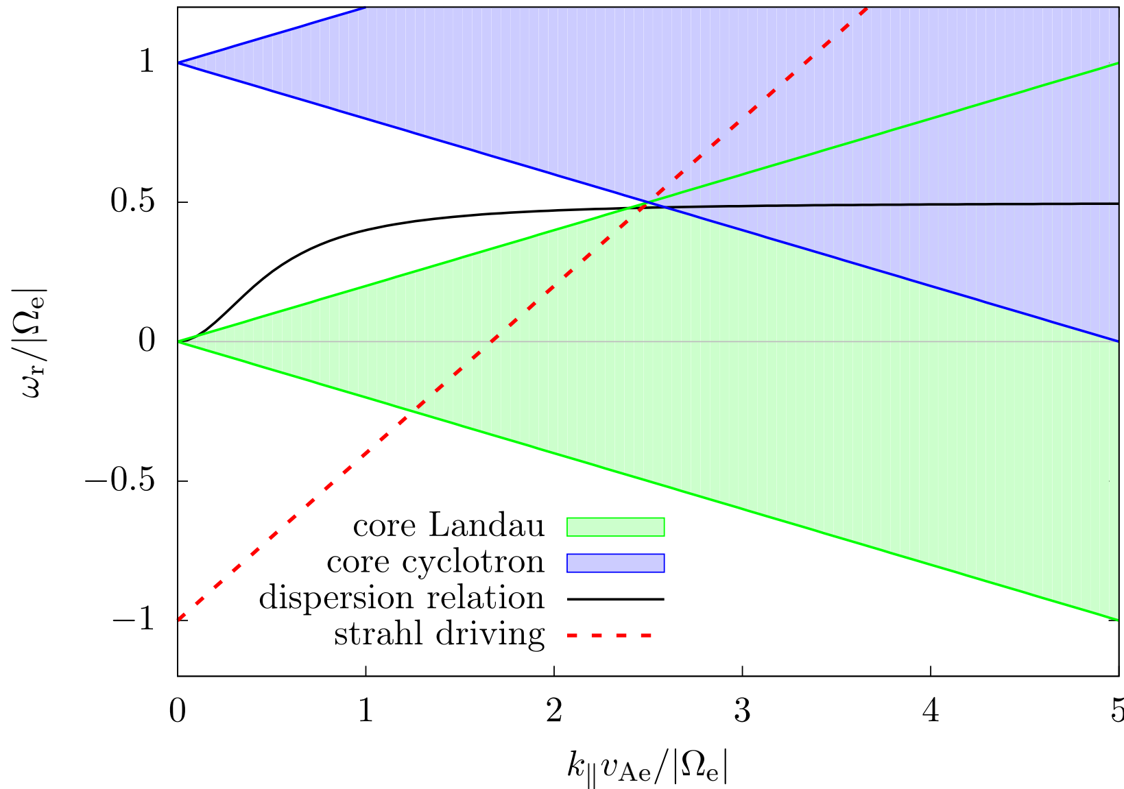
Figure 3. Dispersion relation and resonance conditions for the FM/W mode with \theta = 60^\circ in regime 2. The black line shows Equation (14). The blue and green areas show Equations (16) and (17), respectively, and the red line shows Equation (13) with U_s = 3w_c . We use w_c = 0.2v_{Ae} . This situation represents a marginally stable state for the FM/W instability.
