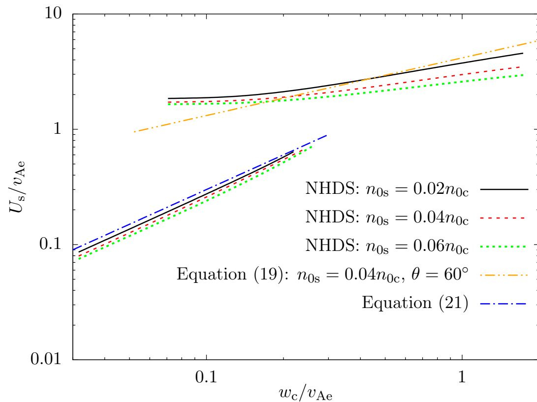
Figure 4. Comparison of Equations (19) and (21) with numerical solutions of the hot-plasma dispersion relation from our NHDS code. The orange and blue lines show Equations (19) and (21), except that the \gtrsim -signs have been replaced with equal-signs. We use w_s = 2w_c and T_{0p} = T_{0c} . For the numerical solutions, we show isocontours of constant maximum growth \gamma_k = 10^{-3}|\Omega_e| with v_{\text{Ap}}/c = 10^{-4} . The analytical solutions use \theta = 60^\circ , while the numerical solutions are evaluated at the angle for which the lowest U_s leads to a maximum growth rate of \gamma = 10^{-3}|\Omega_e| .
