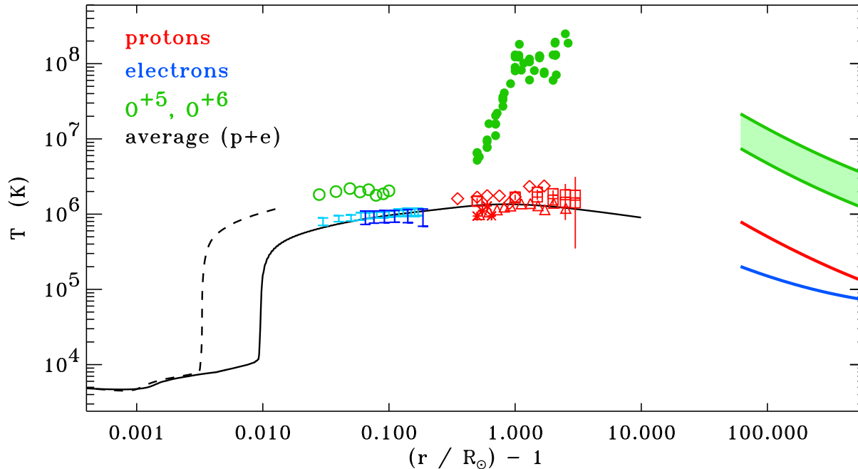
Figure 6: Radial dependence of empirical and model temperatures in polar coronal holes and fast w streams. Mean plasma temperatures from a semi-empirical model (dashed black curve; Avrett and Loe 2008 ) and from a turbulence-driven coronal heating model (solid black curve; Cranmer et al., 2007 ). from off-limb SUMER measurements made by Wilhelm (2006) (dark blue bars) and Landi (2008) (li blue bars), T_p from UVCS measurements assembled by Cranmer (2004b) (see text), and perpendicular C ion temperatures from Landi and Cranmer (2009) (open green circles) and Cranmer et al. (2008) (fil green circles). In situ proton and electron temperatures in the fast wind ( r > 60 R_\odot ) are from Cranmer et al. (2009) .
