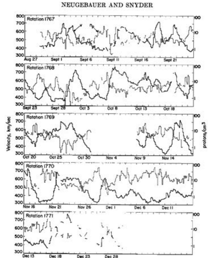
Fig. 5. 3-hour average values of plasma velocity v and proton number density n_p (logarithmic scale) versus time. The time base is chosen to show the 27-day-recurrence features associated with solar rotation.
