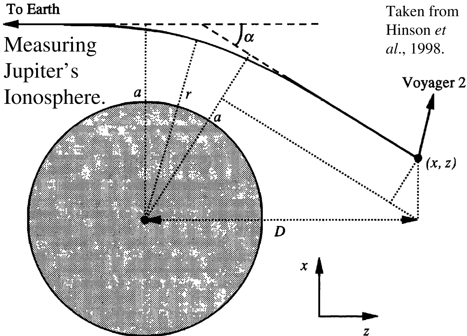
Figure 1. Schematic of Voyager 2 occultation by Jupiter. Solid line shows “ray path” followed by radio signals propagating from spacecraft to Earth. Impact parameter a , radius at ray periapse r , and spacecraft-to-planet distance D are measured from the local center of curvature of Jupiter, which is also the coordinate origin.
