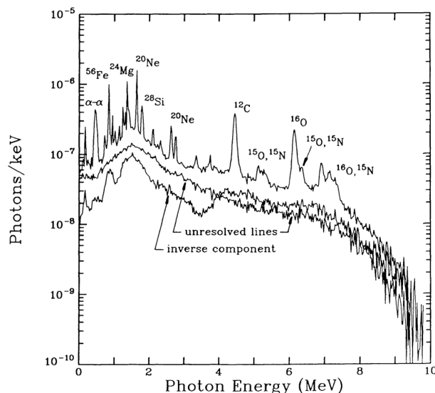
FIG. 1.—Theoretical solar flare nuclear de-excitation gamma-ray spectrum
