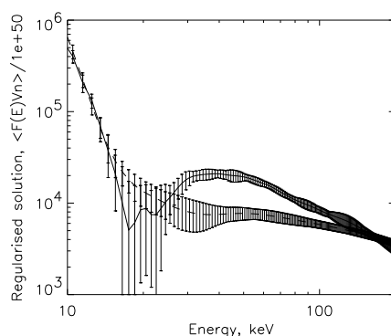
Fig. 8. Inverted mean electron flux of the August 20, 2002 solar flare for the time interval 08:25:20- 08:25:40 UT. The dash line shows the spectra with albedo correction. The confidence intervals represent the range of solutions found by allowing the incident photon spectrum to range randomly within the estimated (instrument + shot noise) errors.
