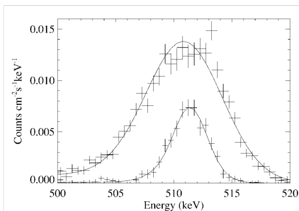
FIG. 3.—Count spectra of the solar 511 keV annihilation line (instrumentally broadened) derived by subtracting bremsstrahlung and nuclear contributions during the October 28 flare when the solar line was broad (11:06–11:16 UT) and narrow (11:18–11:30 UT). The solid curve is the best-fitting model that includes a Gaussian line and positronium continuum.
